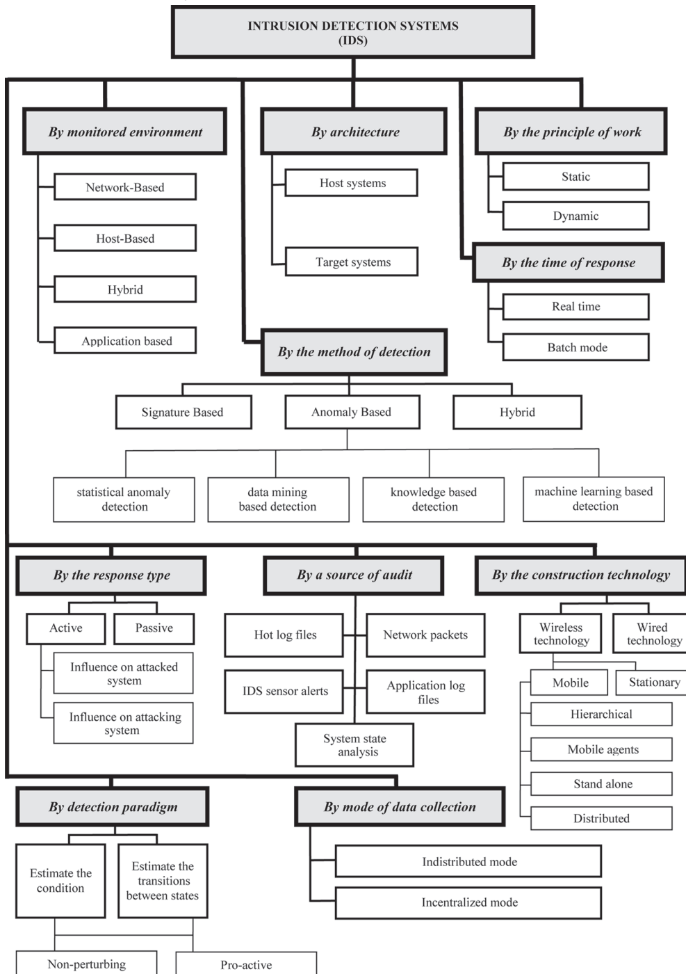
Draw. 12. IDS classification in accordance with modern trends in information system
