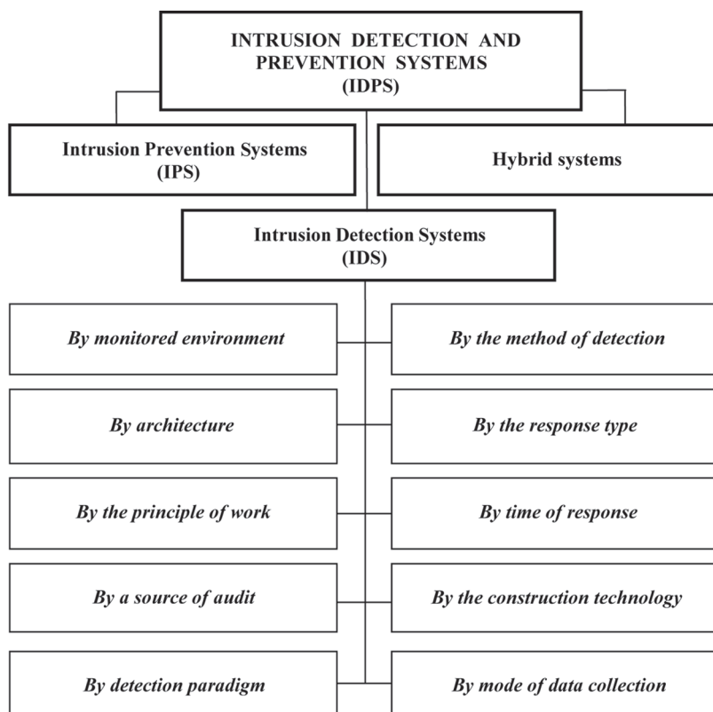
Draw. 1. Classification features of the intrusion detection system taxonomy
